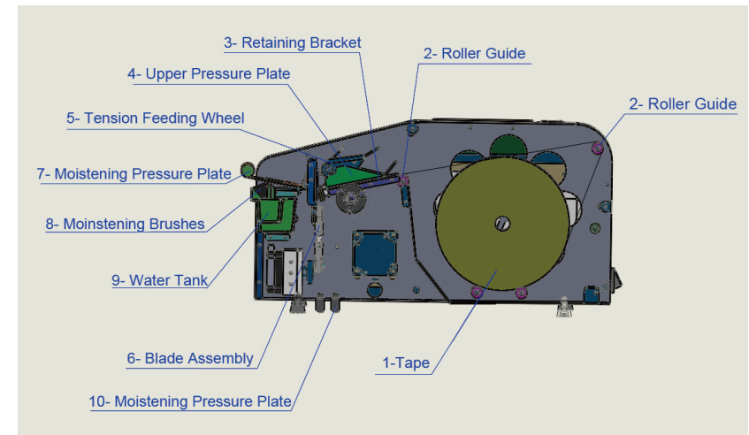
Figure 1: Illustration of the Machine
