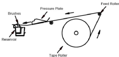
Figure 7: Introduction Diagram for Placing the Tape Roller
